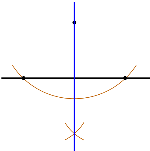
Perpendicular line through a point off the line.
