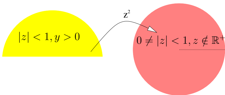
FIGURE 27. Another conformal mapping illustration.
