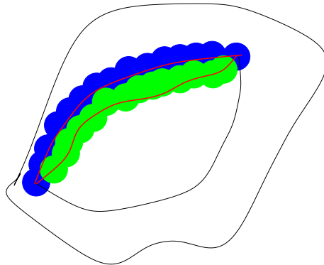
FIGURE 14. The monodromy theorem.
