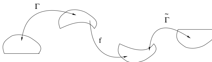
FIGURE 31. Analytic continuation across an analytic arc.
