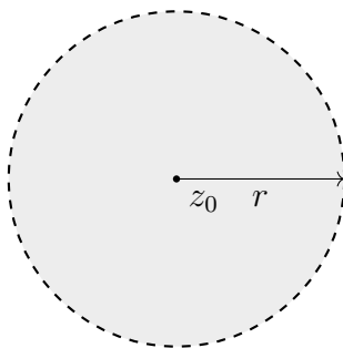
FIGURE 50. Open disk \mathbb{D}(z_0, r) = \{z : |z - z_0| < r\} : boundary dashed to indicate exclusion.
