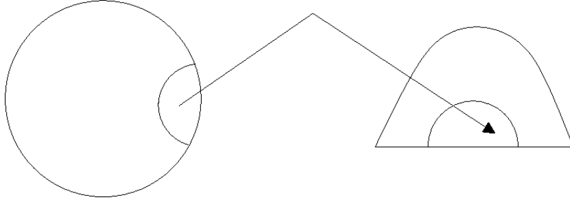
FIGURE 30. Boundary behavior across line segments.
