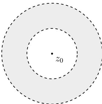
FIGURE 53. Annulus \{z : r < |z - z_0| < R\} : region between two excluded boundary circles.
