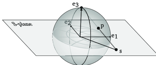
FIGURE 40. The Riemann sphere (taken from Google images)
