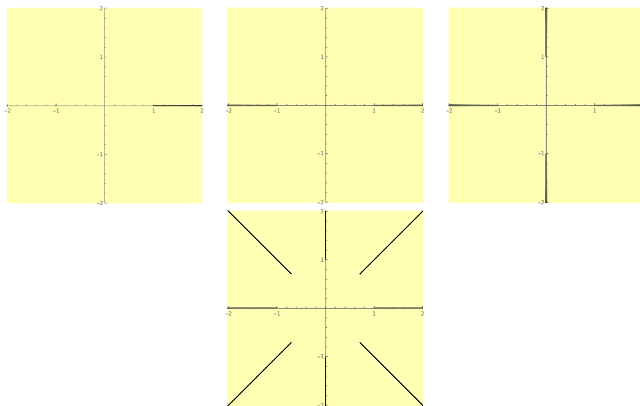
FIGURE 23. \mathbb{C} with one, two, four, and eight symmetric cuts. More generally, the directions of the cuts can be taken along the roots of unity \omega_1, \dots, \omega_k , k \in \mathbb{N} .
