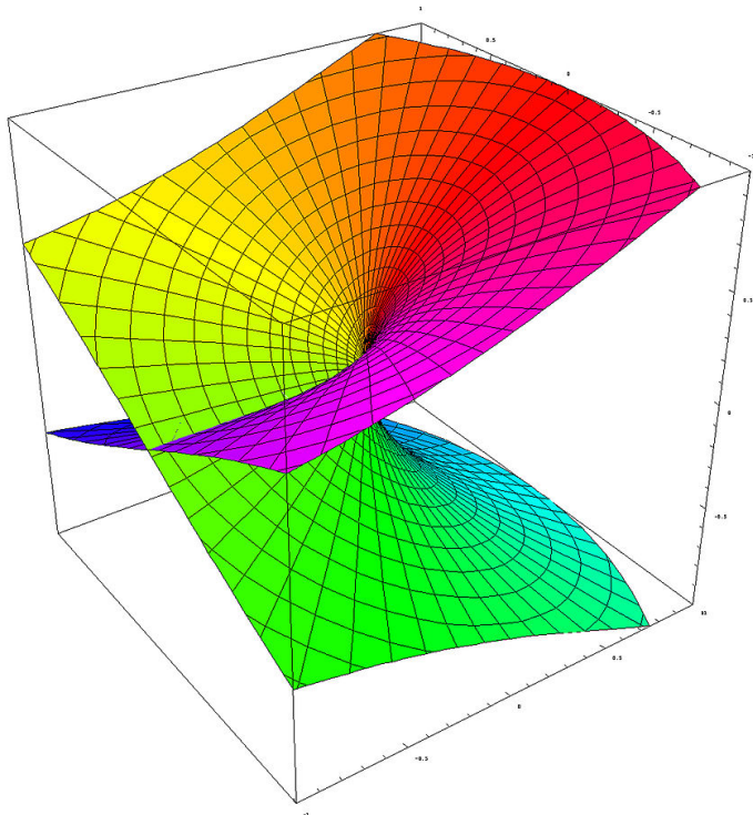
FIGURE 42. An approximate depiction of the Riemann surface of the square root (from https://commons.wikimedia.org/wiki/ )
