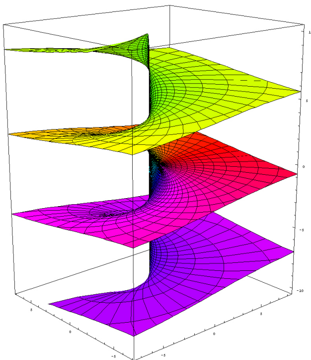
FIGURE 41. The Riemann surface of the log (from https://en.wikipedia.org/wiki/Complex_logarithm )
