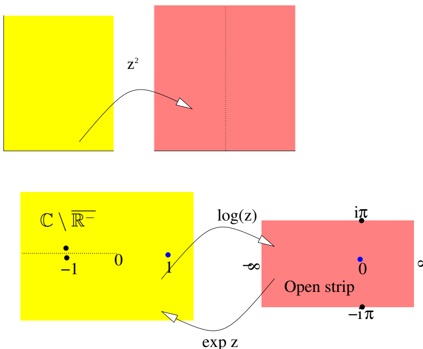
FIGURE 25. A conformal mapping example.
