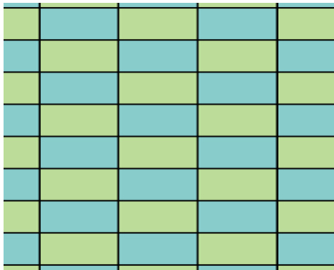
FIGURE 32. Tiling by reflections of a rectangle.
