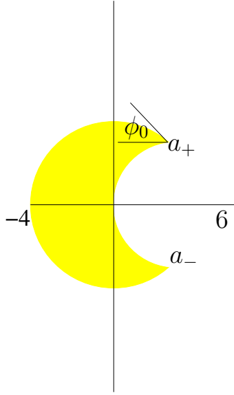
FIGURE 28. Mapping a crescent-shaped domain to a half-plane.
