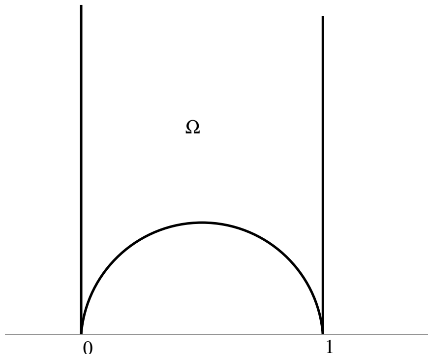
FIGURE 45. The domain \Omega
