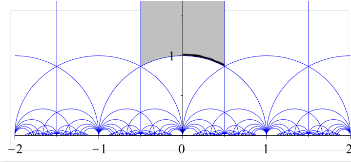
FIGURE 43. The fundamental region \mathcal{R} (the grey region together with the right part of the circle, that is, starting at i ) and the action of PSL(2, \mathbb{Z}) on it, figure from Wiki: [15].
