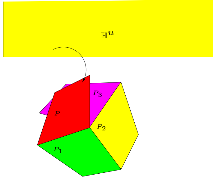
FIGURE 37. Successive reflections.
