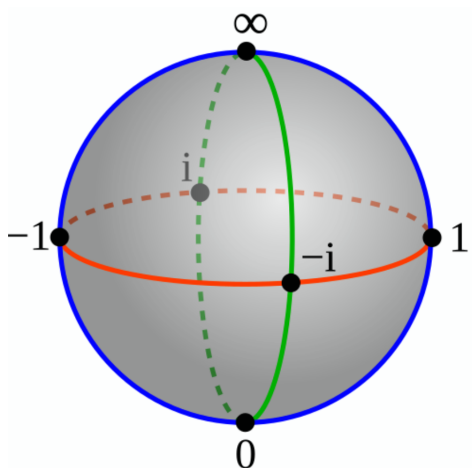
FIGURE 21. The Riemann sphere (adapted from Wikimedia Commons).
