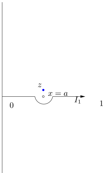
FIGURE 48. Analyticity of \Phi when \phi is analytic in a neighborhood of \mathcal{C} .
