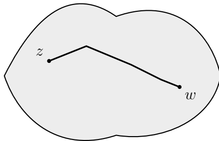
FIGURE 54. Any two points in a domain can be joined by a polygonal path (Proposition 48.19).
