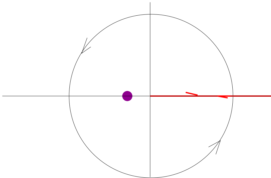
FIGURE 19. Contour for the evaluation of (26.2).
