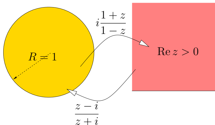
FIGURE 26. Mapping between a circle and a half-plane.
