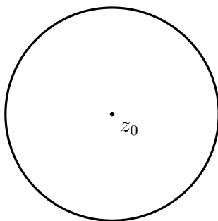
FIGURE 52. Boundary of the disk: the circle |z - z_0| = r .
