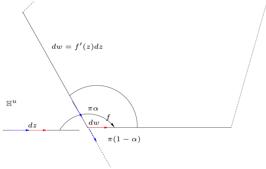
FIGURE 36. Schwarz-Christoffel transformations: two adjacent sides of the polygon.
