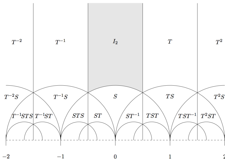
FIGURE 44. Marked action of S, T
