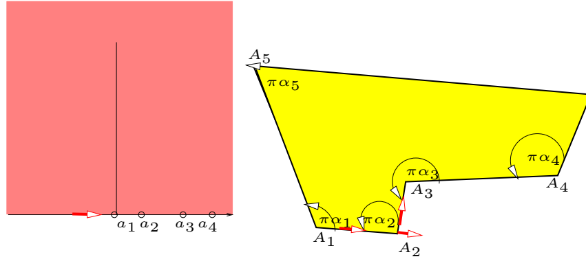
FIGURE 35. Schwarz-Christoffel transformations: a closed polygon.
