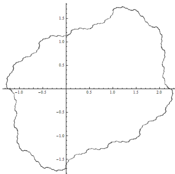
FIGURE 34. The conformal image of the unit disk under the map G .
