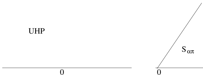
FIGURE 22. The map z \mapsto z^{1/\alpha} maps the open sector of opening \pi\alpha conformally onto the open upper half-plane. The boundary point 0 maps to 0, and the upper boundary of the sector is rotated to -\mathbb{R} .
