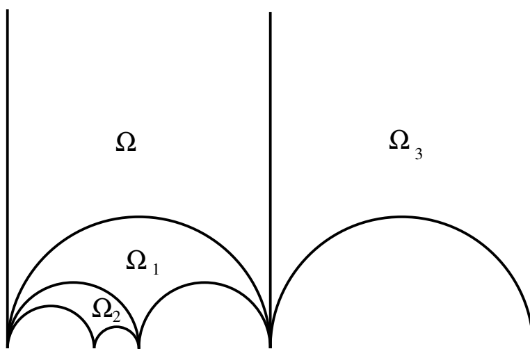
FIGURE 46. Successive reflections
