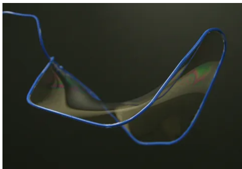
FIGURE 7. A soap film (image from the google images, https://math.hmc.edu/~jacobsen/demolab/soap-film-2/ )
