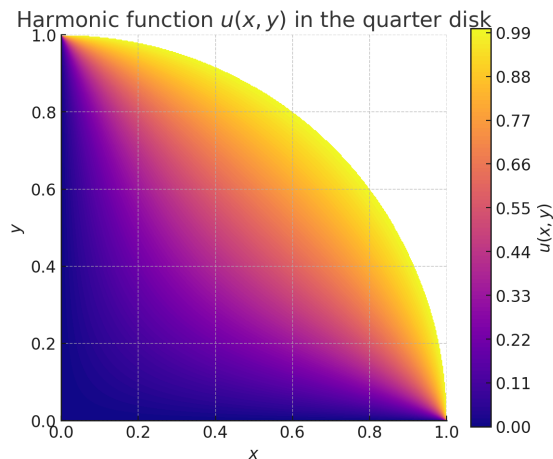
FIGURE 29. Color density plot of the heat equation solution for a quarter disk
