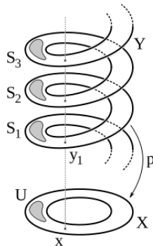
FIGURE 20. The covering space of an annulus (adapted from Wikimedia Commons).
