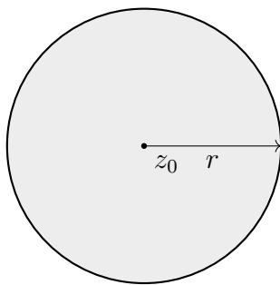
FIGURE 51. Closed disk \overline{\mathbb{D}}(z_0, r) : solid boundary indicates inclusion.
