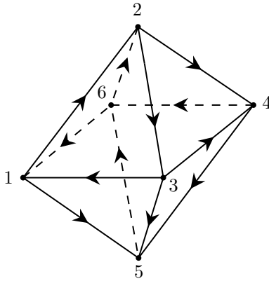
FIGURE 2. The octahedron version of (6.1-a). Four mutually non-adjacent faces correspond to \mu = \text{Re } \omega and the remaining four to \text{Im } \omega , where seven faces (all but one of the latter, namely, 531) represent the same orientation of the boundary surface. The four \mu -faces are also characterized by being coherently oriented by the arrow-marked orientations of their sides.
