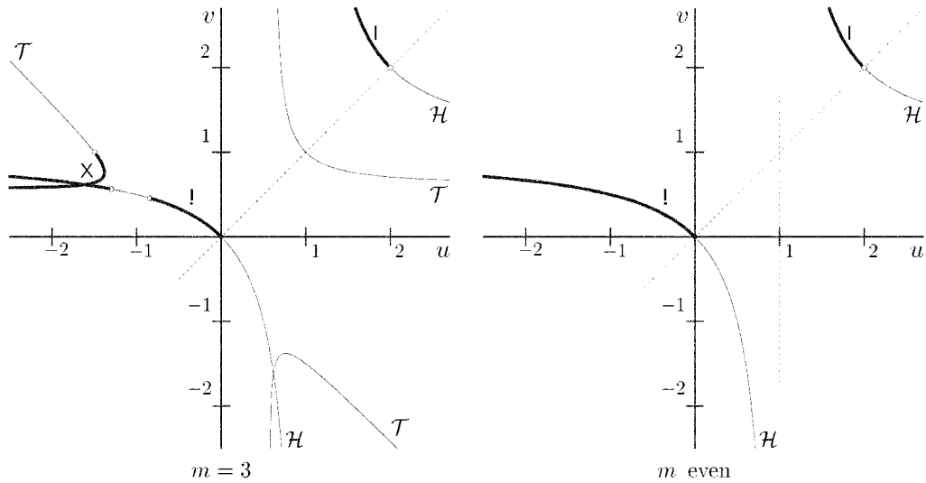
FIGURE 1. The components !, l of \mathcal{C} and, for odd m , the two beams of X , are the thick curve segments, each contained in \mathcal{H} except for the \mathcal{T} -beam of X , contained in \mathcal{T} . For m = 3 , the set \mathcal{T} consists of the isolated point (0, 0) and three disjoint real-analytic curves in \mathbb{R}^2 , diffeomorphic to \mathbb{R} . (See Remark 30.5.)
