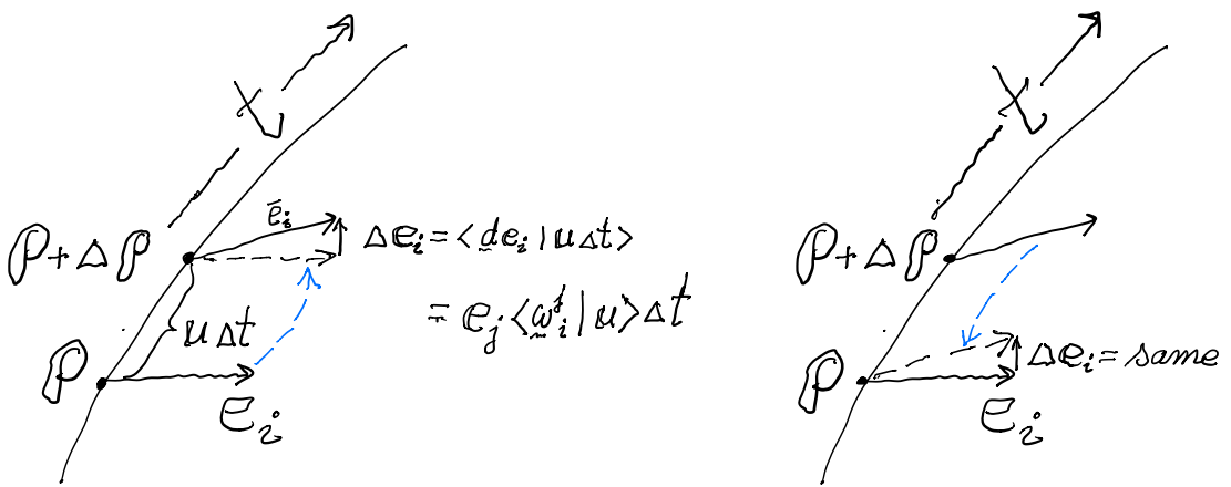
Figure 30.1: Along a t -parametrized curve a preexisting t -parametrized family of basis vectors deviates from being parallel.
