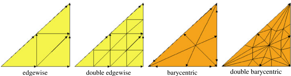
Fig. 4 Simplicial subdivisions of \Delta[2]
