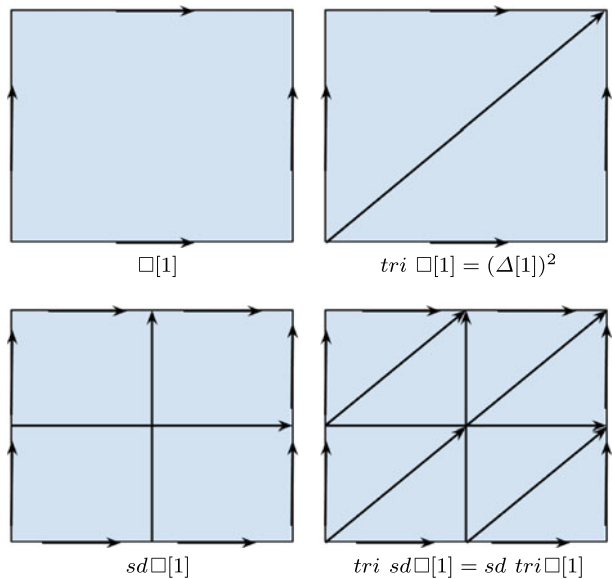
Fig. 2 Edgewise subdivision, a cubical analogue, and triangulation
