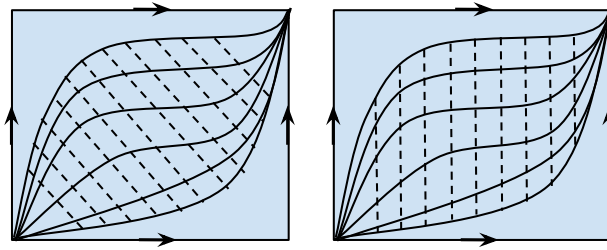
Fig. 3 Weak ( left ) and strong ( right ) types of directed homotopies. The homotopies on both sides are identical up to reparametrization of paths. Only the right homotopy is monotone in the homotopy coordinate, traced by the dotted lines . For compact quadrangulable streams, the equivalence relations generated by weak and strong definitions of directed homotopy are equivalent [Theorem 8.13]
