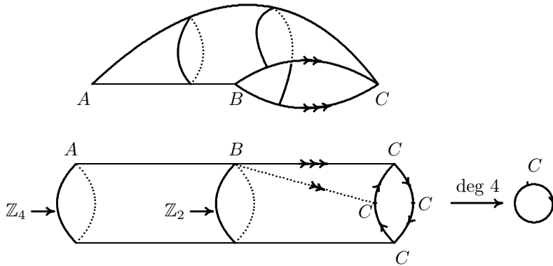
FIGURE 2. 2-skeleton of the quotient space G \setminus \mathbb{R}^3 . The four side faces of the polyhedron P fold up into the two adjacent cylinders. On the right, the boundary circle of the cylinder gets attached to the circle by a degree 4 map. The top and bottom faces of P get identified into a single square, which attaches to the cylinder as indicated. The two loops in the cylinder based at A, B have isotropy \mathbb{Z}_4 and \mathbb{Z}_2 respectively. All remaining points have trivial isotropy.
