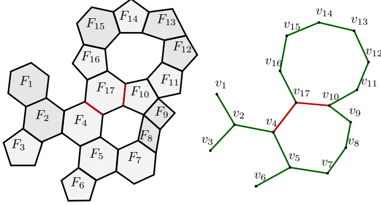
FIGURE 3. Non-contractible region, its dual graph G , a spanning tree T for G (green edges), enumeration of the vertices, and corresponding enumeration of the faces (Section 4.3).
