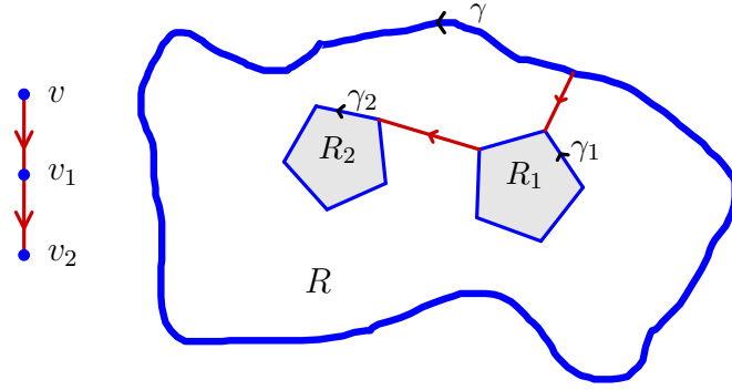
FIGURE 4. Graph B of blue loops and red edges associated to the non-contractible region R (Section 4.5).
