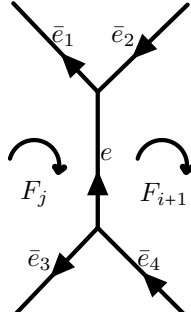
FIGURE 21. Local picture near the edge e (Lemma 5).
