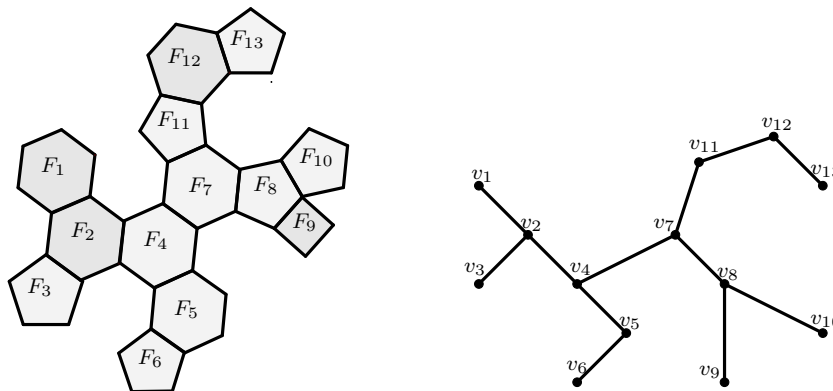
FIGURE 2. Contractible region, its dual tree T with an enumeration of its vertices, and corresponding enumeration of the faces (Section 4.3).
