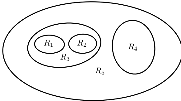
FIGURE 1. Example of enumeration of regions (Section 4.2).
