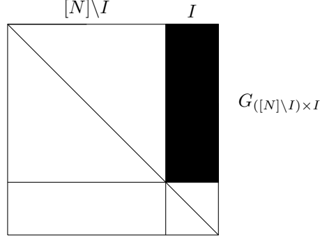
FIGURE 2. Decomposition into i.i.d. parts.
