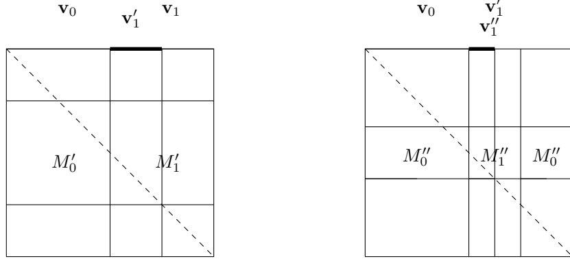
FIGURE 4. Finding non-structured subvectors.
