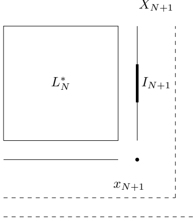
FIGURE 3. Row and column exposure process during reshuffling.
