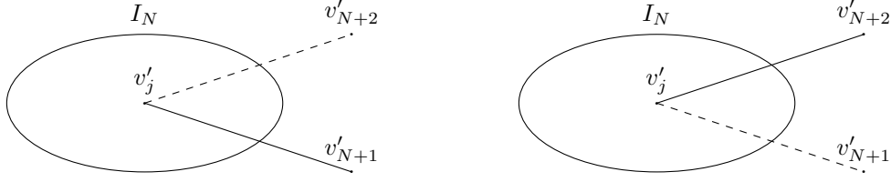
FIGURE 1. Swapping neighbors.
